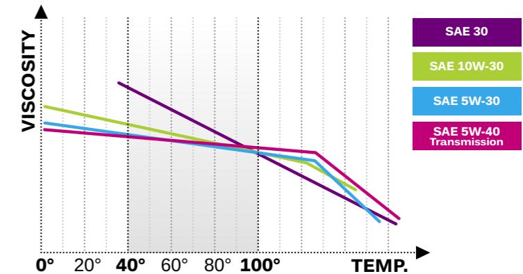
Viscosity performance
