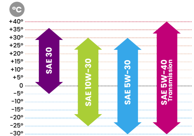
Temperature performance
